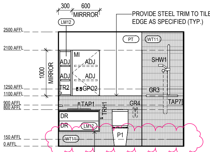
ILA BT-07 ELEVATION 1 Scale 1 : 50
