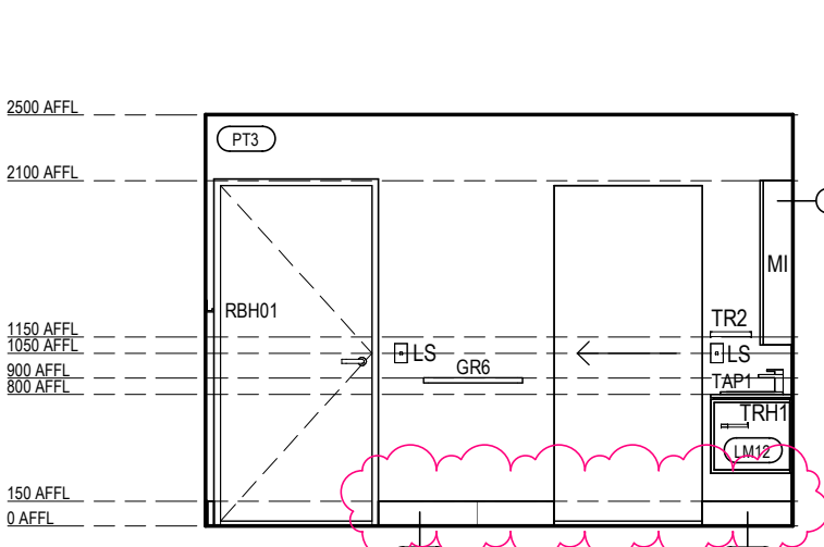
ILA BT-07 ELEVATION 2 Scale 1 : 50
