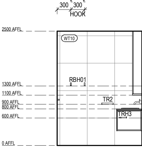
ILA BT-08 ELEVATION 2 Scale 1 : 50
