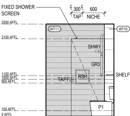
ILA BT-09 ELEVATION 2 Scale 1 : 50
