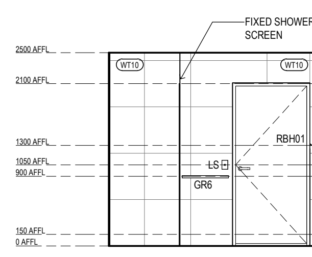
ILA BT-08 ELEVATION 3 Scale 1 : 50
