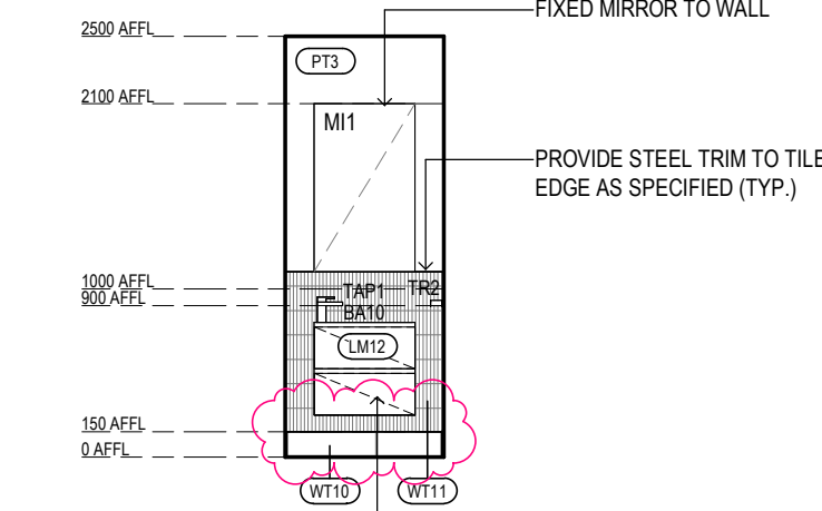
ILA PD-01 ELEVATION 4 Scale 1 : 50
