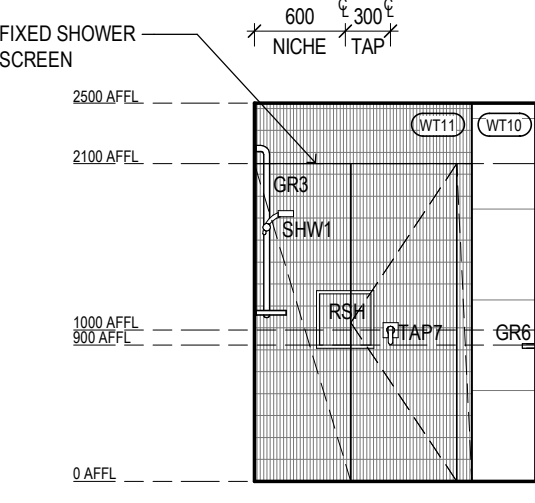
ILA BT-08 ELEVATION 4 Scale 1 : 50
