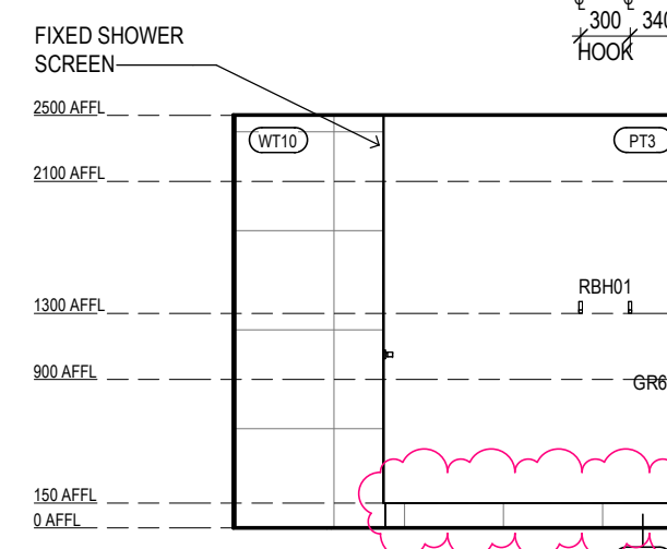
ILA BT-07 ELEVATION 3 Scale 1 : 50
