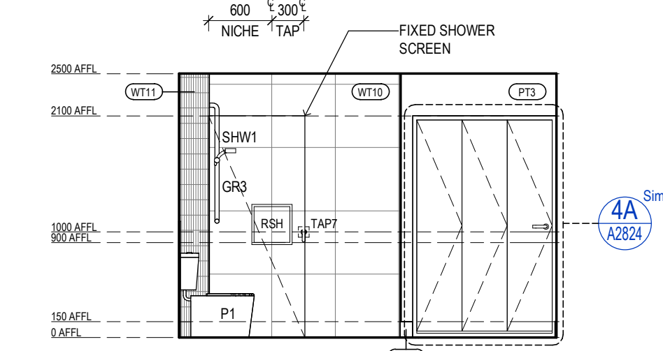
ILA BT-07 ELEVATION 4 Scale 1 : 50
