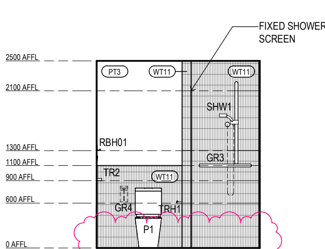
ILA BT-06 ELEVATION 1 Scale 1 : 50
