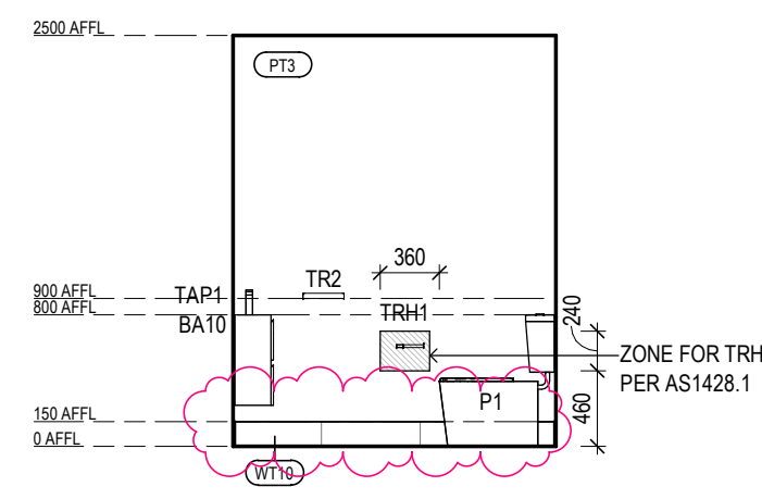
ILA PD-01 ELEVATION 3 Scale 1 : 50
