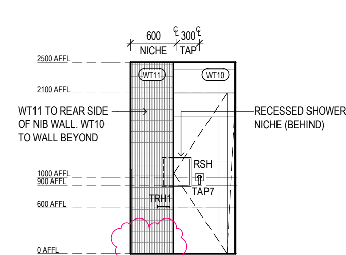
ILA BT-06 ELEVATION 4 Scale 1 : 50
