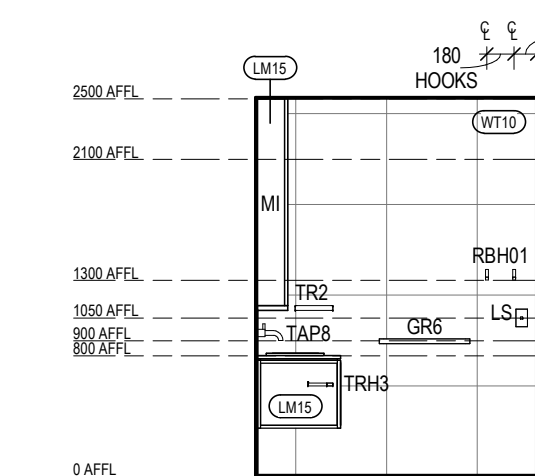
ILA BT-09 ELEVATION 4 Scale 1 : 50
