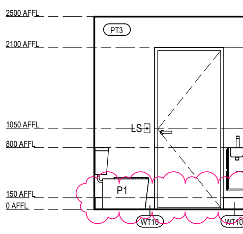
ILA PD-01 ELEVATION 1 Scale 1 : 50
