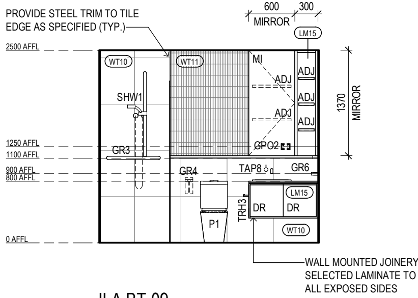
ILA BT-09 ELEVATION 1 Scale 1 : 50
