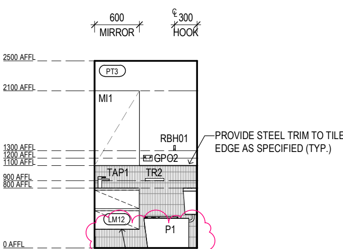
ILA BT-06 ELEVATION 2 Scale 1 : 50
