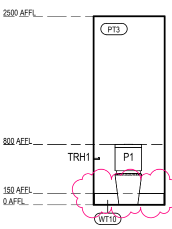
ILA PD-01 ELEVATION 2 Scale 1 : 50
