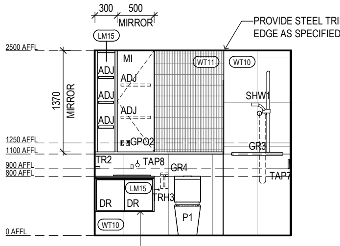
ILA BT-08 ELEVATION 1 Scale 1 : 50
