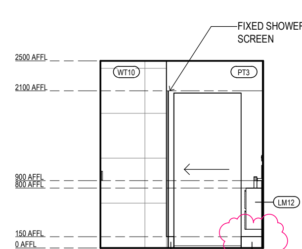
ILA BT-06 ELEVATION 3 Scale 1 : 50
